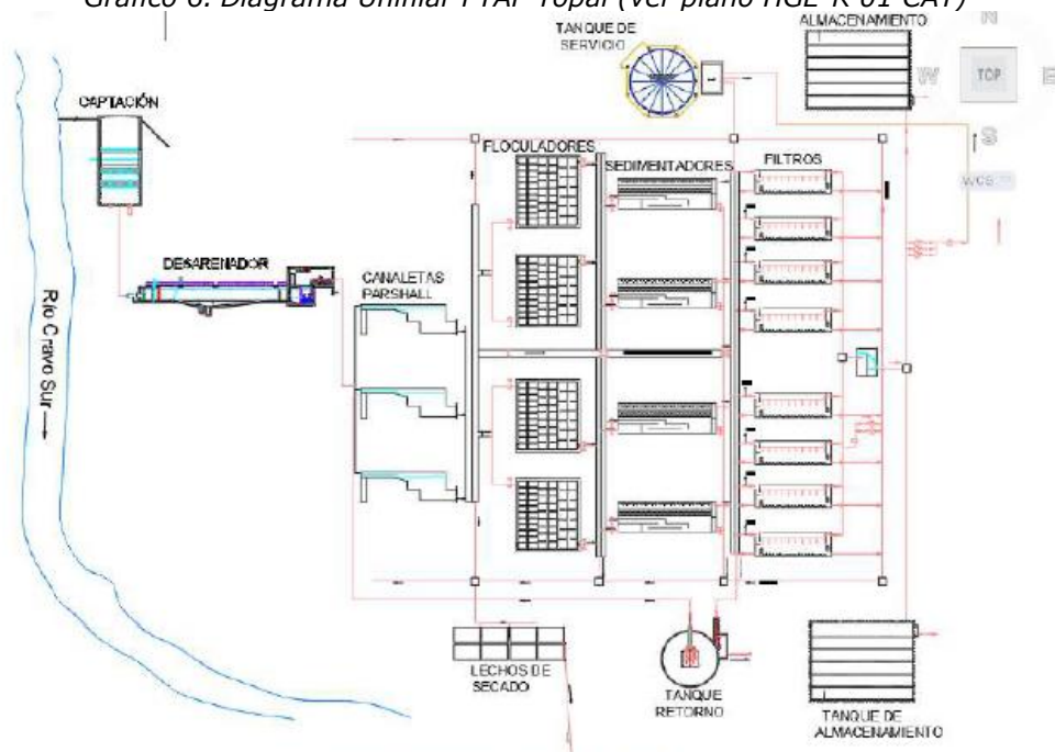
Grafico 6. Diagrama Unifilar PTAP Yopal (ver plano HGE-R 01 CAY)
